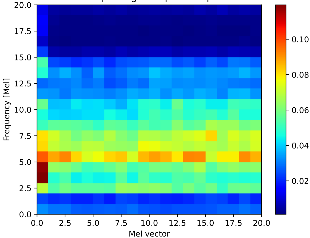
MEL Spectrogram np#helicopter
